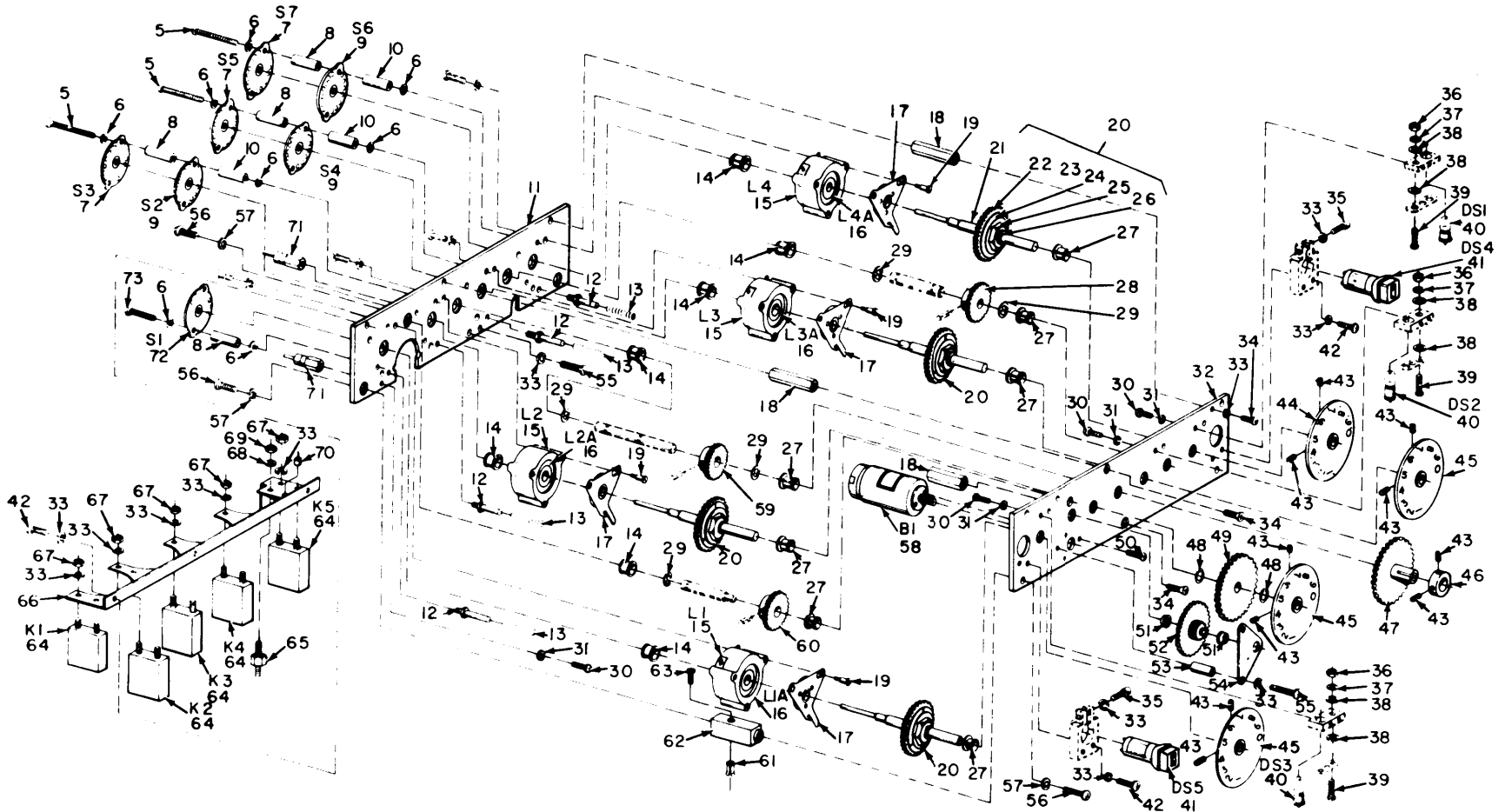
EXPLODED VIEW
