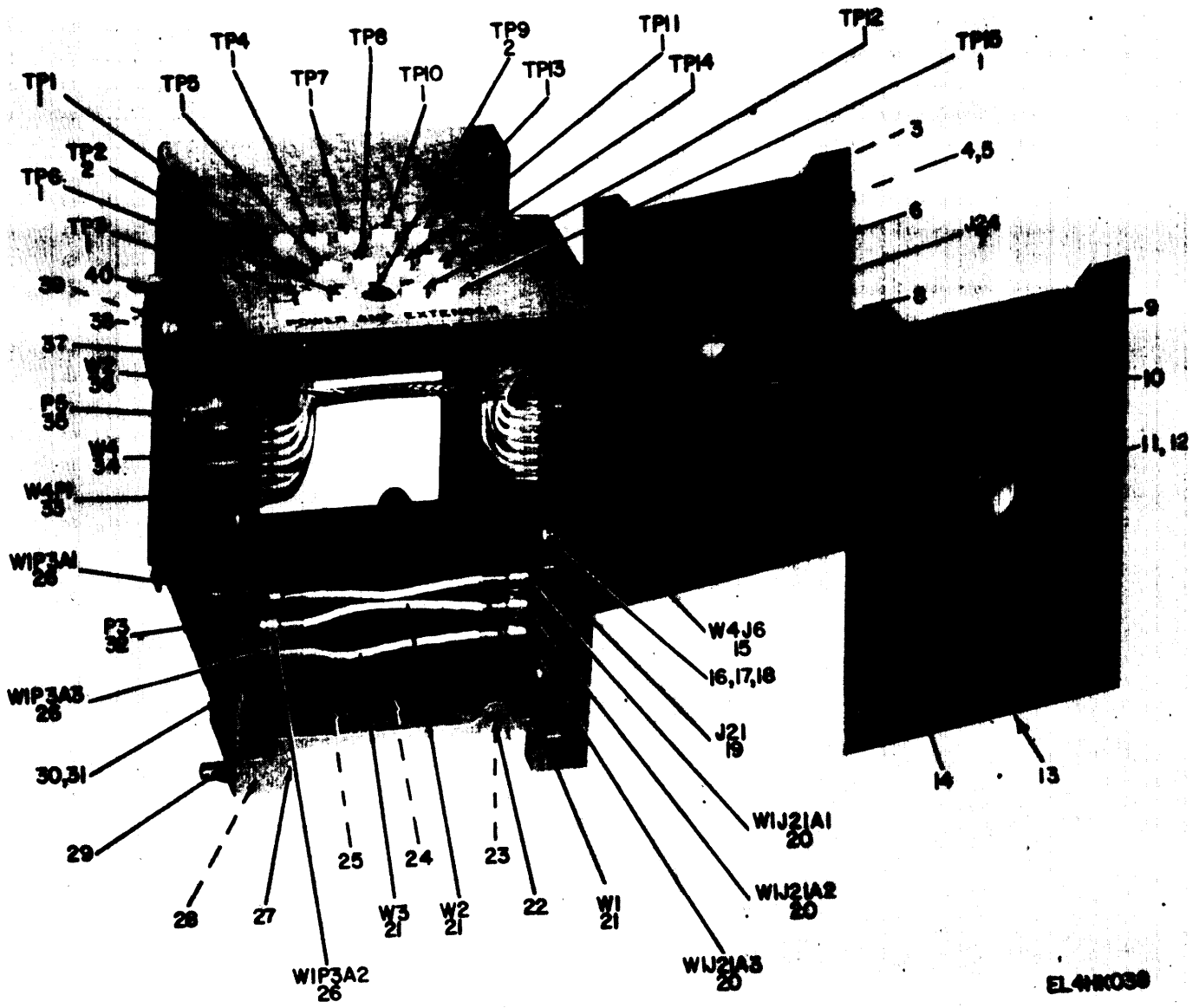
Figure 17. Extender, Module MX-4911/ARC-51X.
