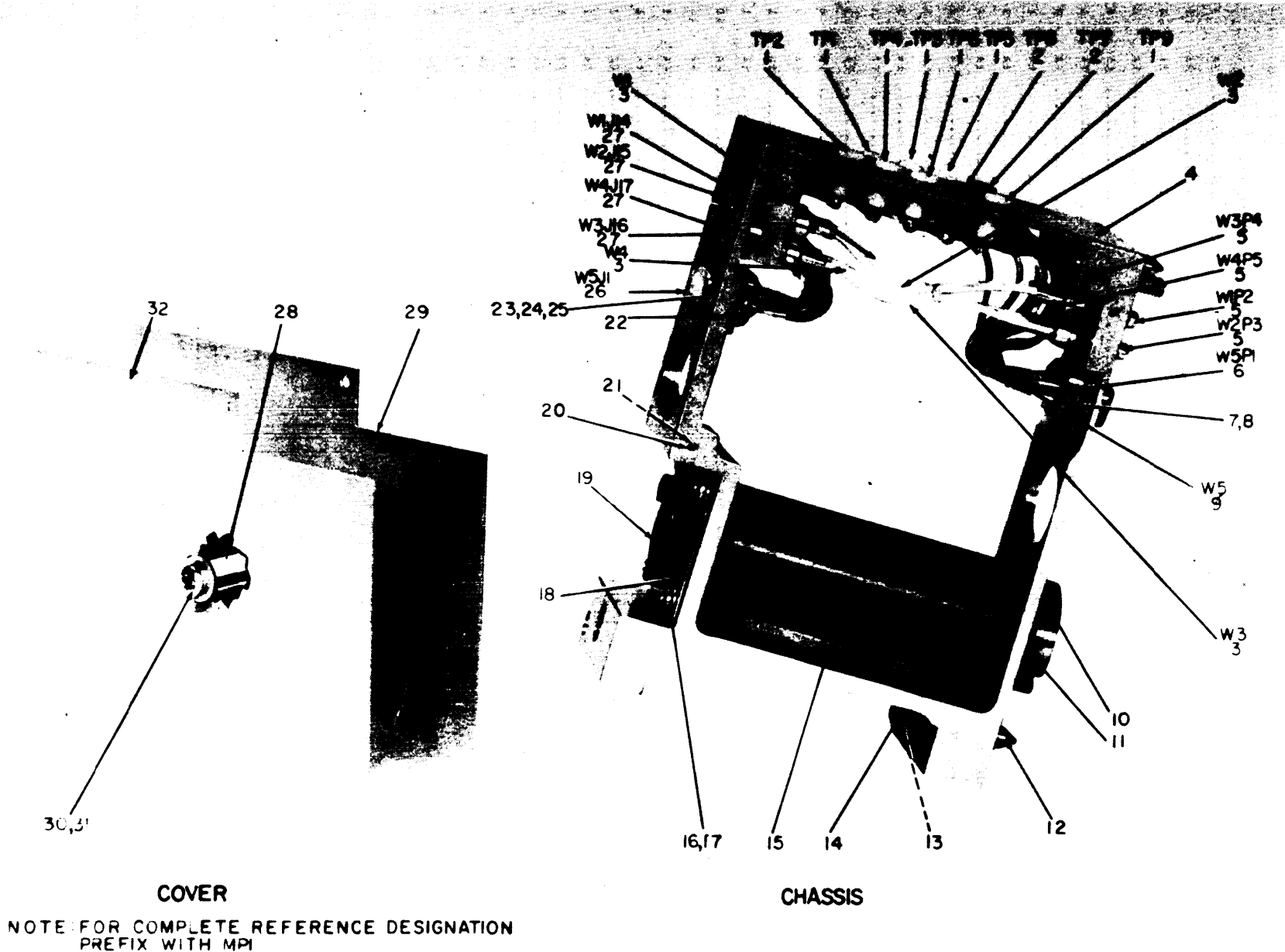
Figure 22. Extender, Module MX-4906/ARC-51X.
