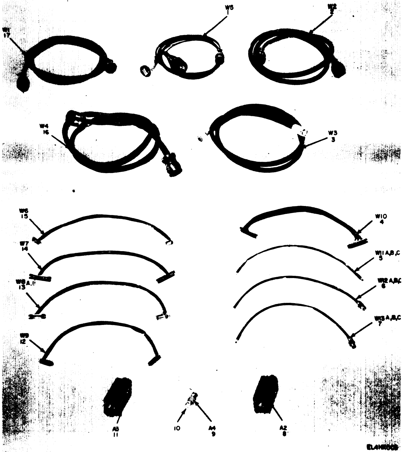
Figure 3. Maintenance Kit, Electronic Equipment MK-731/ARC-51X and MK-731A/ARC-51X, Cable Assemblies and Adapters.
