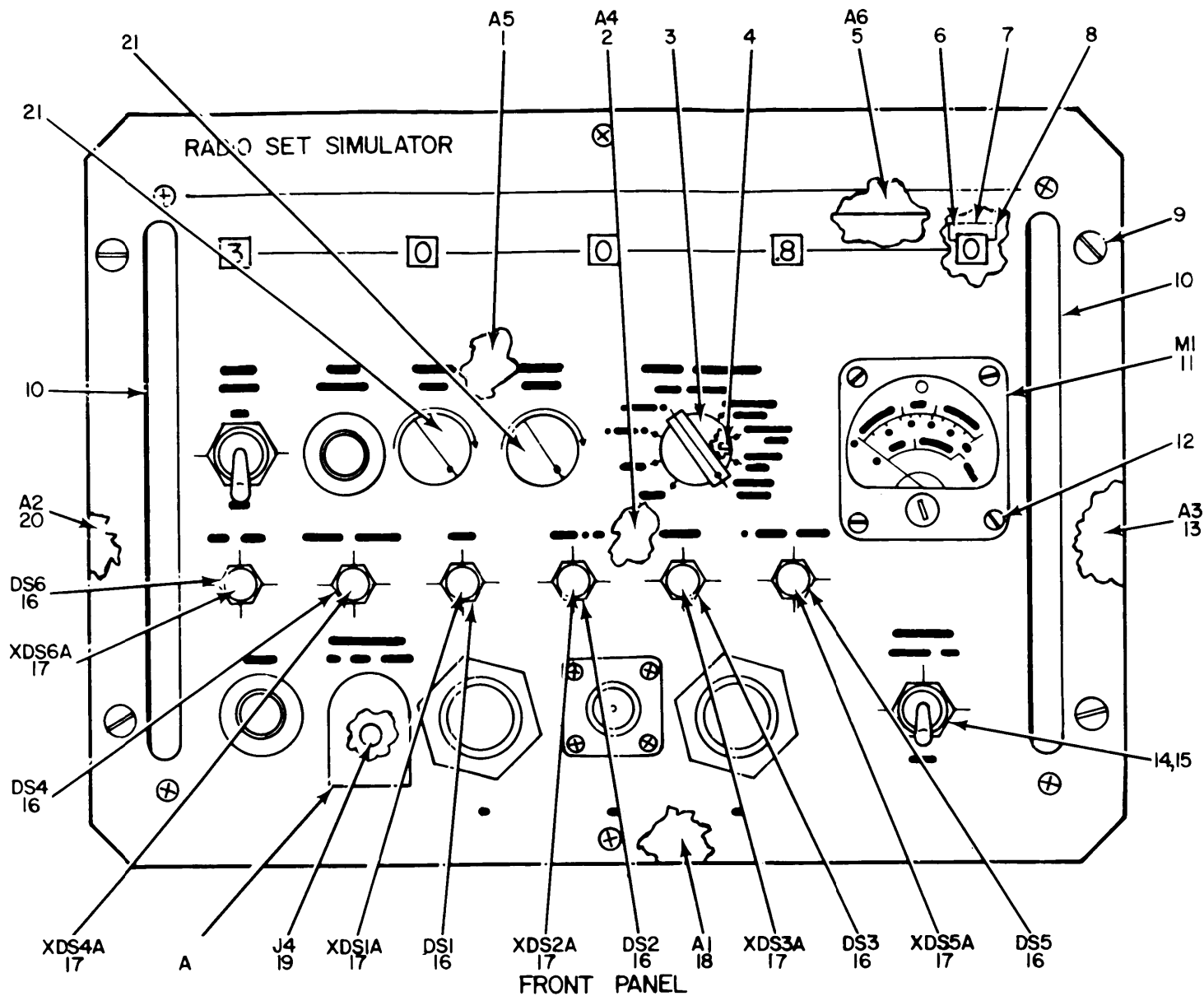
Figure 5. Simulators, Test Set, Radio SM-348/ARC-51X and SM-348A/ARC-51X.
