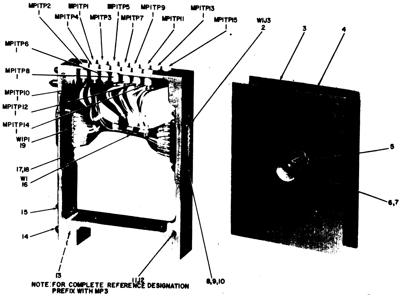
Figure 20. Extender, Module MX-4908/ARC-51X.
