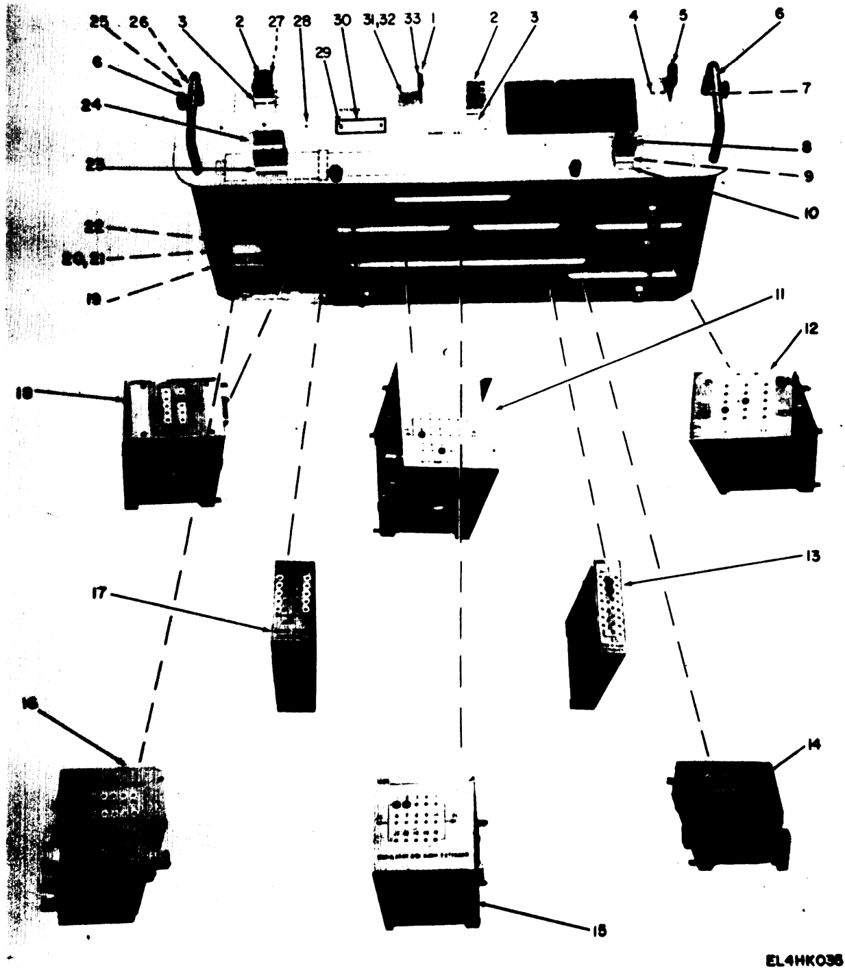
Figure 14. Mounting Tray, Module Extender MT-3372/ARC-51X.
